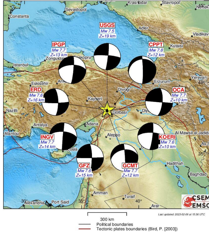
Moment Tensor map of earthquake: Mag: 7.5 2023-02-06 10:24:49 UTC Lat: 38.11 Lon: 37.24 Depth: 10.0 km
